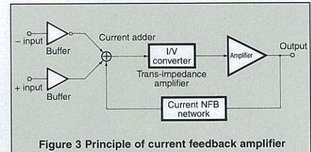
Figure 3 Principle of current feedback amplifier
